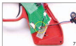
Remove Battery/Solenoid Harness
