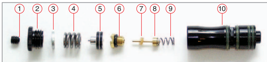
Low-Pressure Regulator
