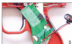
Flip Board To Expose Wiring
