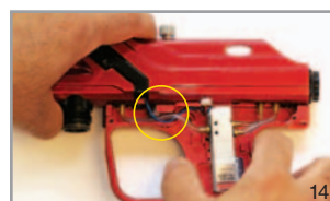
Slide Frame Back From Body
