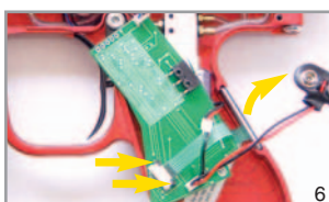
Lift Up LCD Ribbon Locks
