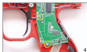
Remove Board Retaining Screws
