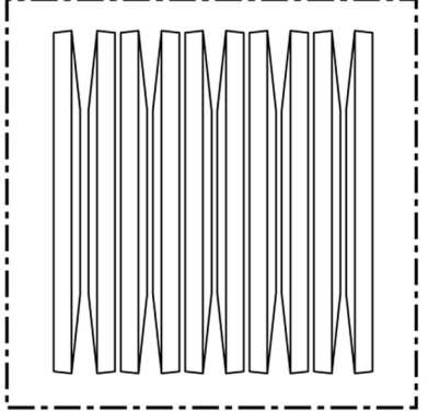
★ FIGURE 2 SPRING PACK BELLEVILLE WASHER DETAIL
