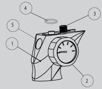
Vertical Adapter Assembly - SHKNXT105
