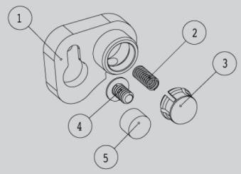
FIG. 21 → BALL DETENT ASSEMBLY
